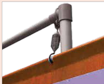
The top of the graphics is also held with springs, the springs also help make the graphics taut & gives greater flexibility with graphics size
